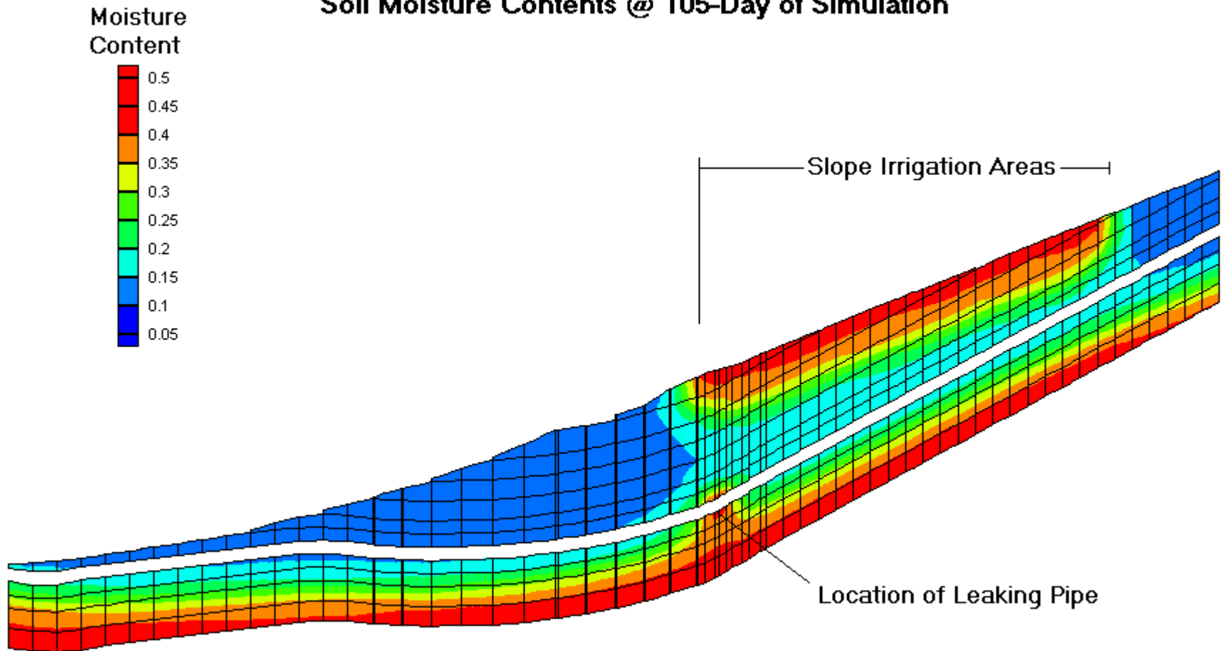
Soil Moisture Contents @ 105-Day of Simulation
