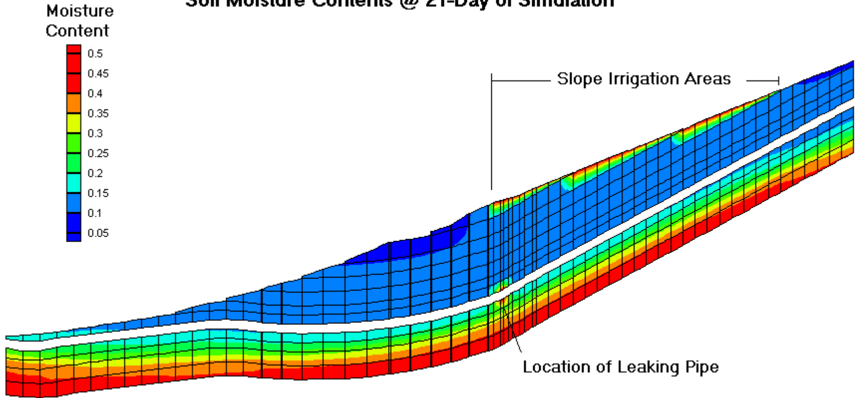
Soil Moisture Contents @ 21-Day of Simulation
